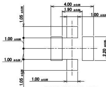
MASK THICKNESS : t=0.12 METAL MASK
