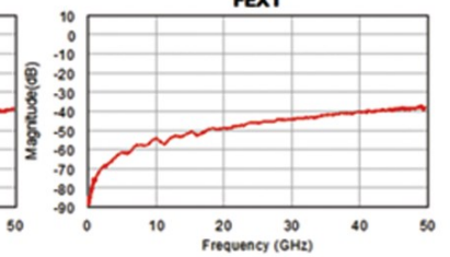
FEXT
